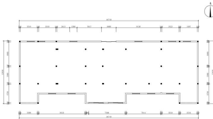
FIG 29 Original structure of Building 1 : 120 (Author's self drawn)
