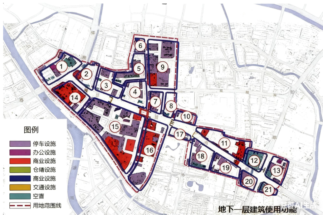
Figure 2-1 Functional distribution of underground space along Yanling West Road, Changzhou
