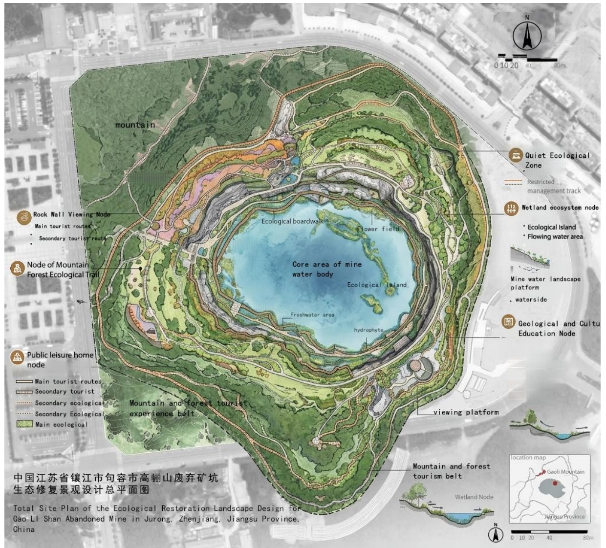
Figure A16 Total Site Plan of the Ecological Restoration Landscape Design for Gaolishan Abandoned Mine in Jurong, Zhenjiang, Jiangsu Province, China
