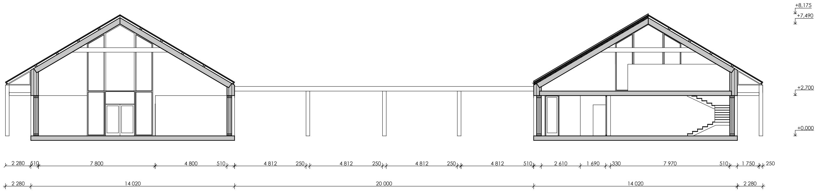
Section 1
